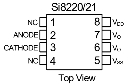
Figure 17. Pin Configuration
